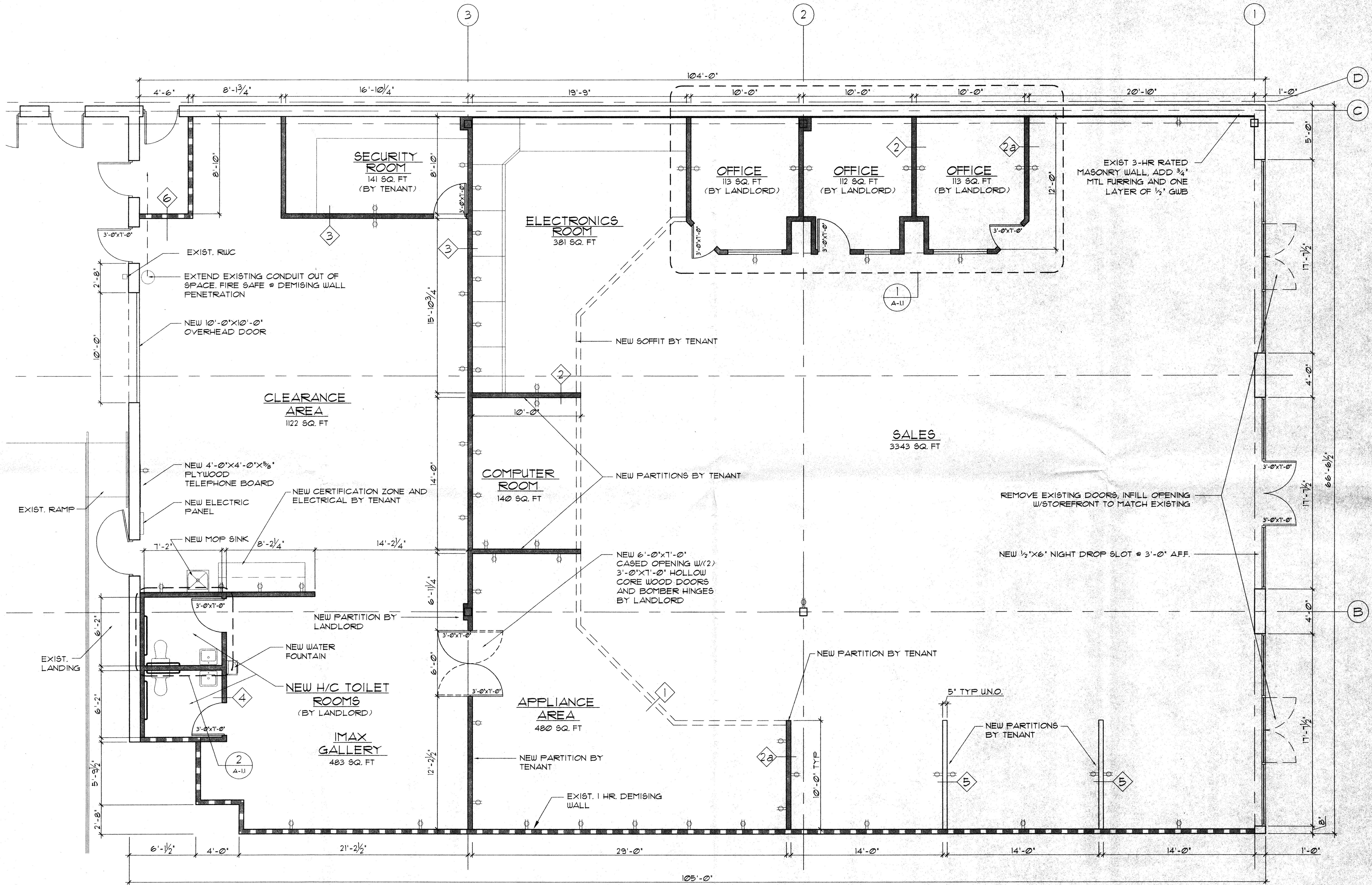
1 FLOOR PLAN A-10 SCALE: 1/4"=1'-0"
